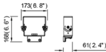
65/872 Trunnion Mount
