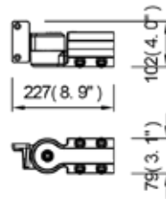
Included 2 3/8" Slip-Fitter
