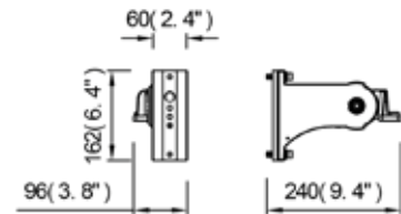
65/870 Universal Mount
