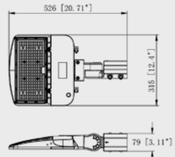
2 3/8" Slip-Fitter (Included)
