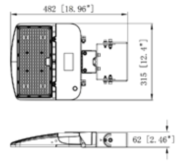
65/872 Trunnion Mount
